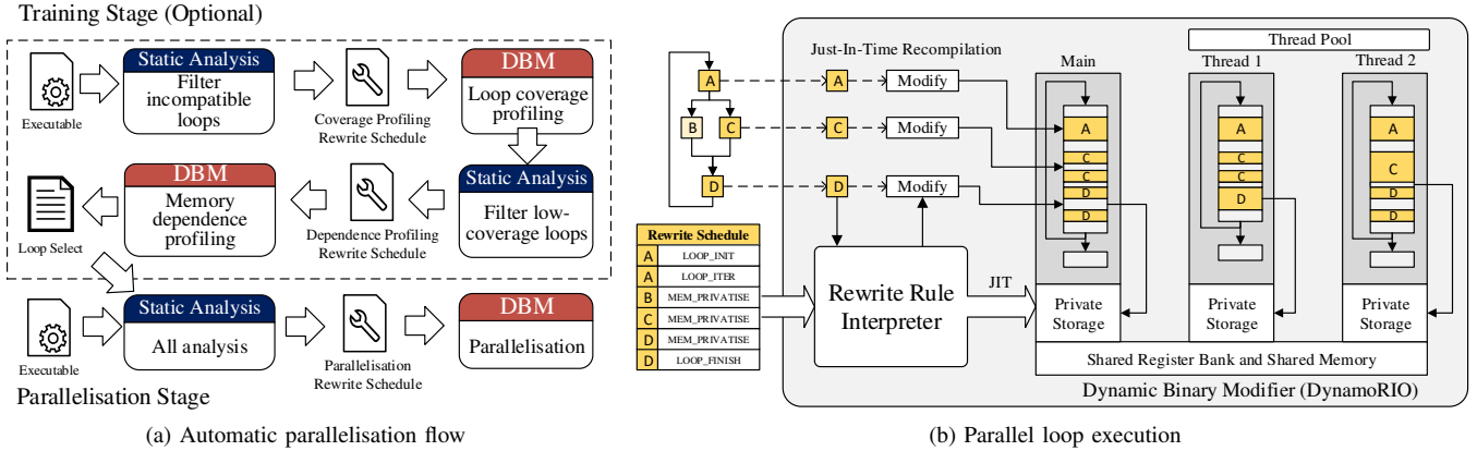
(a) Automatic parallelisation flow (b) Parallel loop execution Fig. 1. Automatic parallelisation in Janus. Rewrite schedules allow the static analyser to control dynamic modification.
