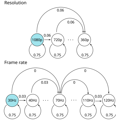
Fig. 8. Transition graphs showing the weights used for the Viterbi algorithm used to control transitions in resolution (top) and frame rate (bottom). The current state of each graph is shown in blue (1080p, 30 Hz). Note that frame rates which deviate by more than 30 Hz from the current state have a transition weight of 0, preventing any such transitions.
