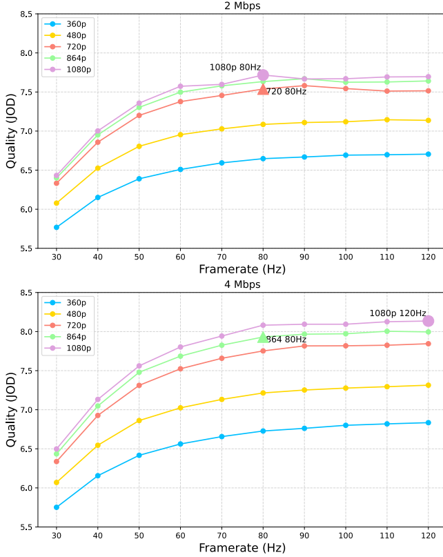
Fig. 4. ColorVideoVDP predictions for the same sequence from the scene “Bistro” rendered at different resolutions and frame rates. The two plots show the results for different bit rates. The resolution and frame giving the highest quality are shown as round markers, and the ones that also reduce the compute cost (computed from Eq. (1)) are shown as triangle markers.
