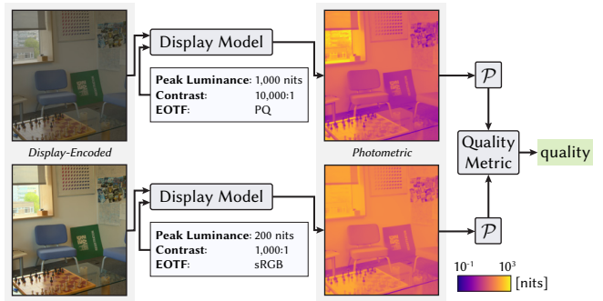
Fig. 1. Metric adaptation strategy . The absolute luminance of HDR reference and tone-mapped test can differ significantly. To accurately predict quality, our display model maps display-encoded content to photometric values, given the specifications of the display. The color map represents the photometric values in \text{cd/m}^2 (nits). Next, a perceptual transfer function, \mathcal{P}(\cdot) , maps these values to a shared display-encoded representation (e.g. 0–1), usable by the quality metric.
