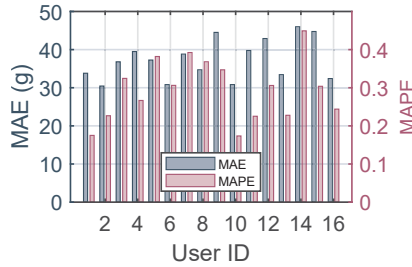
Fig. 12. Impact of different users.
