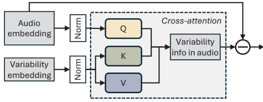
Fig. 7. Cross-attention-based variability disentangle module.
