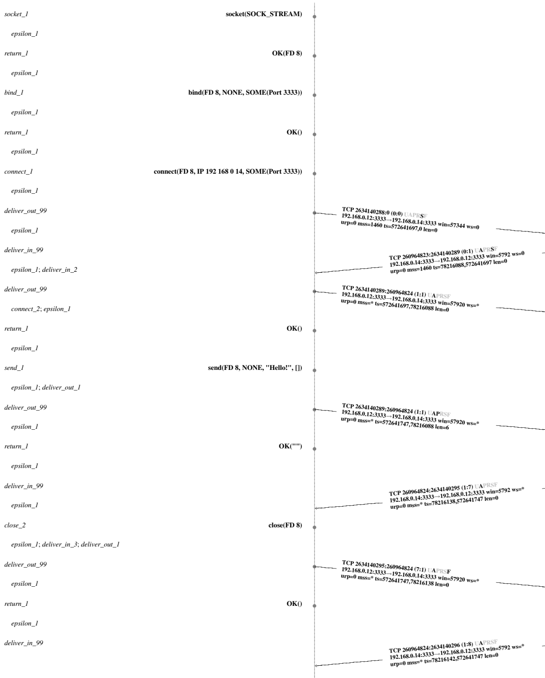
Figure 3. Sample checked TCP trace, with rule firings, but eliding time data – connect() end
