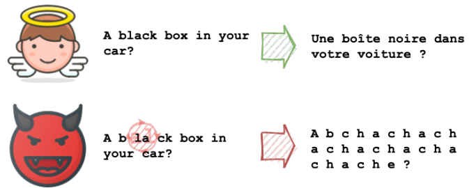
Fig. 3. Attack using reorderings. Example machine translation input is on the left with model output on the right. The red circle denotes the string is encoded in reverse order surrounded by Bidi override characters.
