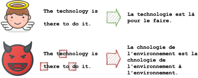
Fig. 1. Attack using invisible characters. Example machine translation input is on the left with model output on the right. Invisible characters are denoted by red boxes, such as between the ‘e’ and ‘t’.
