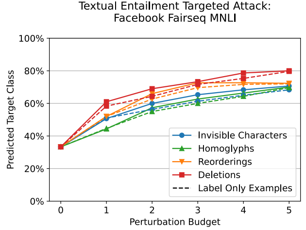
Fig. 11. Targeted accuracy of Fairseq MNLI model with imperceptible perturbations
