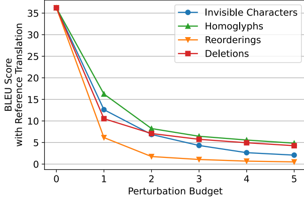
Fig. 6. BLEU scores of imperceptible perturbations vs. unperturbed WMT data on Fairseq EN-FR model
