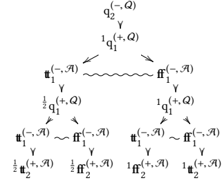
Figure 2. A probabilistic strategy for b : \text{Bool}_1 \vdash M_+ = \text{if } b \text{ (if coin } b \perp) \text{ (if } b \text{ ff } \mathfrak{t}) : \text{Bool}_2
