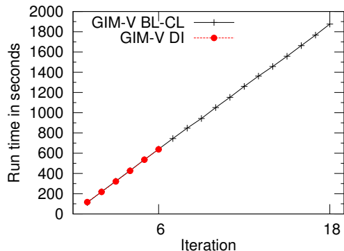
Figure 5. Comparison of GIM-V DI and GIM-V BL-CL for HCC. GIM-V DI finishes in 6 iterations while GIM-V BL-CL finishes in 18 iterations due to long chains.
