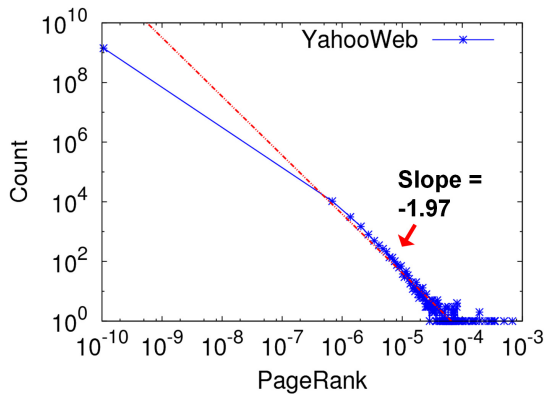
Figure 8. PageRank distribution of YahooWeb. The distribution follows power law with exponent 1.97.
