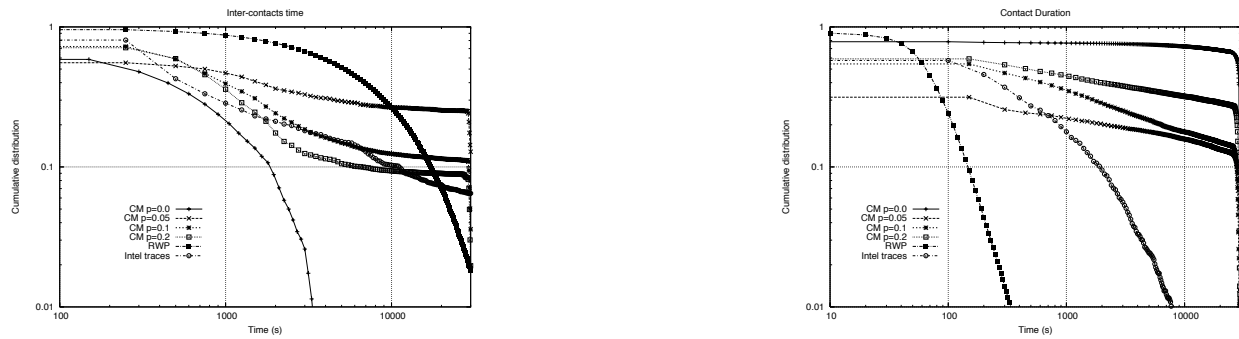
Figure 7: Comparison between synthetic and real traces (log-log coordinates) : (a) cumulative distribution of inter-contacts time in seconds; (b) cumulative distribution of contacts duration in seconds.
