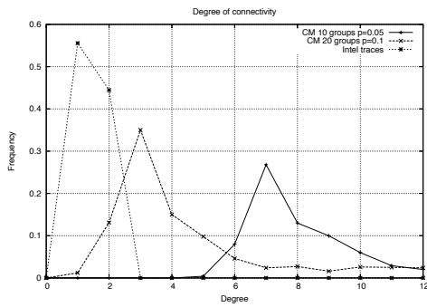
Figure 6: Distribution of the degree of connectivity.
