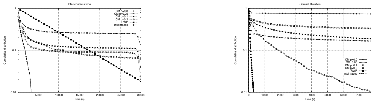
Figure 8: Comparison between synthetic and real traces (semi-log coordinates): (a) cumulative distribution of inter-contacts time in seconds; (b) cumulative distribution of contacts duration in seconds.
