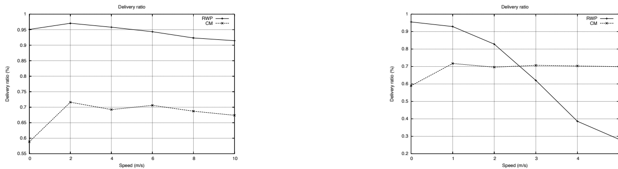
Figure 12: Influence of the mobility model on the protocol performance (delivery ratio vs speed): (a) AODV; (b) DSR.
