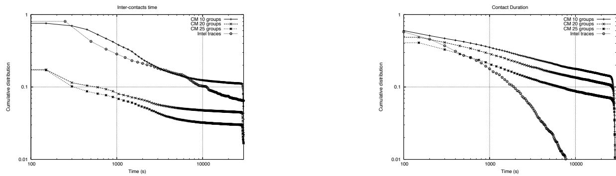
Figure 11: Influence of the number of initial number of groups in input to the network generator based on the Caveman model: (a) cumulative distribution of inter-contacts time in seconds; (b) cumulative distribution of contacts duration in seconds.
