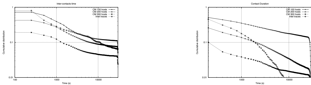
Figure 10: Influence of the density of population: (a) cumulative distribution of inter-contacts time in seconds; (b) cumulative distribution of contacts duration in seconds.
