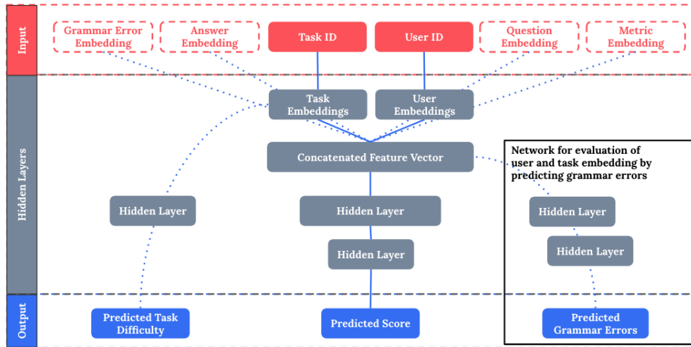
Figure 2: Task score prediction system architecture. Dotted lines and boxes are optional features and network connections.
