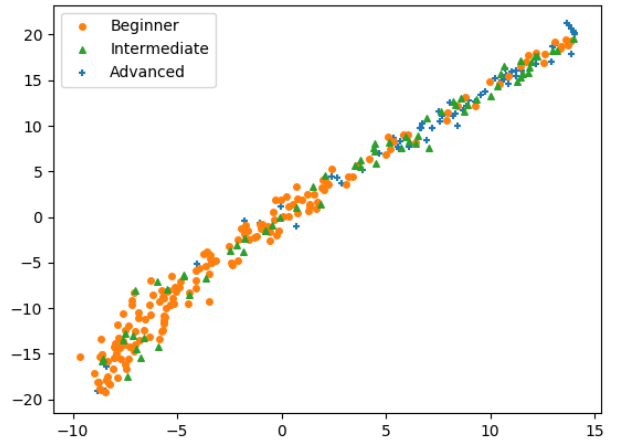
Figure 3: t-SNE of 300 randomly sampled student representations classified by different levels of proficiency
