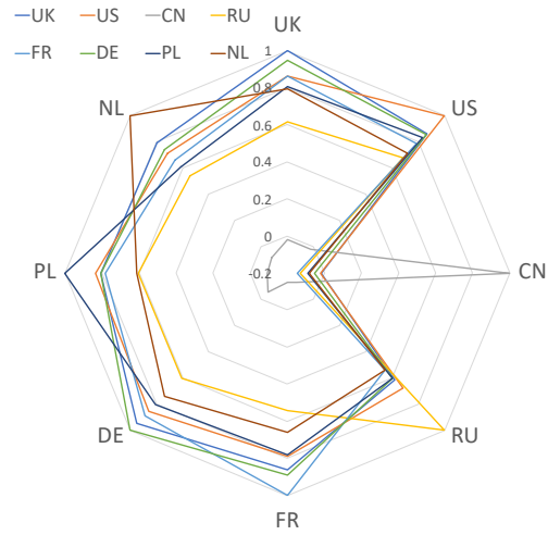
Figure 4: Correlation between numbers of attacks over time between countries, where 1 indicates complete correlation, 0 indicates no correlation, and -1 indicates negative correlation.
