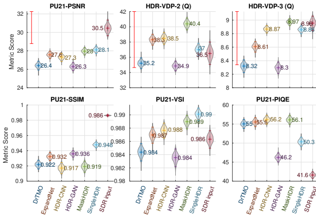
Figure 6: Ranking bootstrapped distributions for SI-HDR methods on the validation dataset. For each distribution, small dashes denote 95% confidence intervals, while the red errors bars show the minimum measurable increment in quality for selected metrics (described in Section 7.4).
