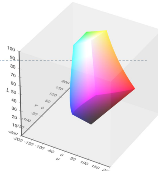
sRGB in CIE L^*u^*v^*
