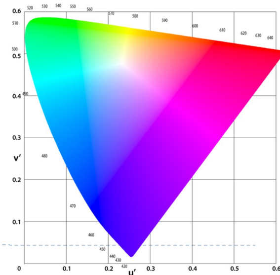
sRGB in CIE L^*u^*v^*
