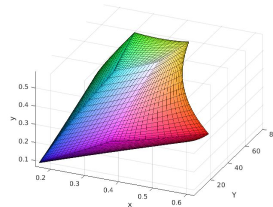
RGB gamut in Yxy colour space
