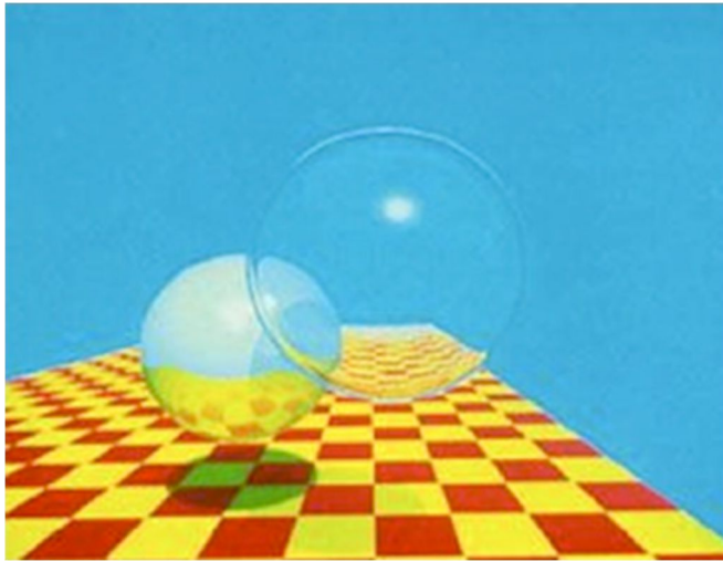
Turner Whitted 1979
