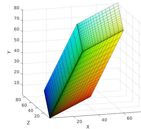
RGB gamut in XYZ colour space
