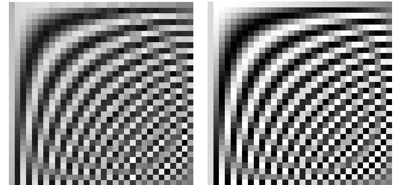
Matrix U' with normalised KLT eigenvector columns
