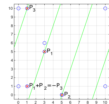
elliptic curve over \mathbb{Z}_{11} ( a = -1, b = 1 )
