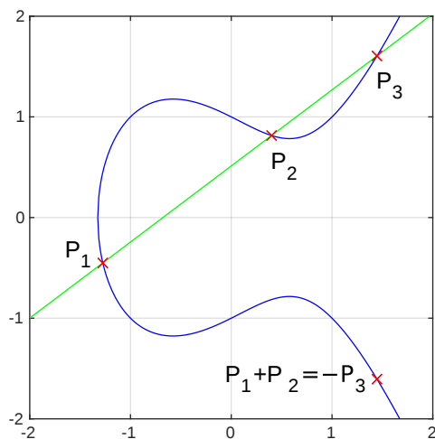
elliptic curve over \mathbb{R} ( a = -1, b = 1 )
