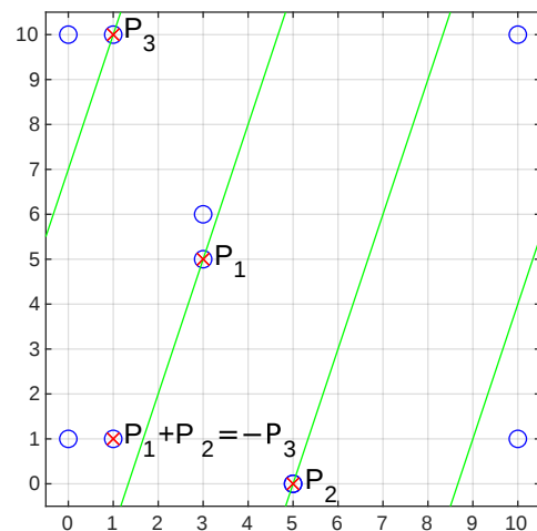
elliptic curve over \mathbb{Z}_{11} ( a = -1, b = 1 )
