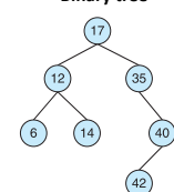
Binary tree
