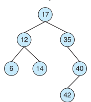
Binary tree
