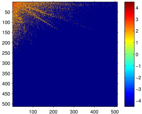
95% truncated 2D DCT (log10)
