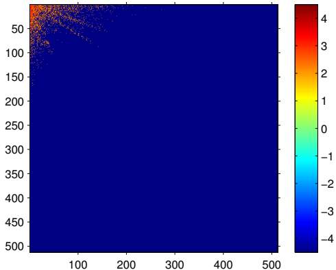
99% truncated 2D DCT (log10)
