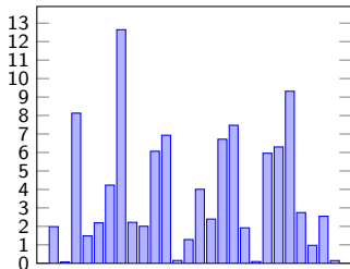
shifted letter freq. (IC=0.065)
