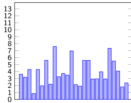
averaged letter freq. (IC=0.046)
