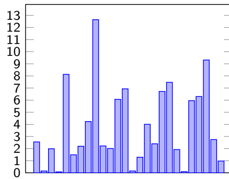
shifted letter freq. (IC=0.065)
