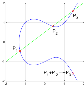
elliptic curve over \mathbb{R} ( a = -1, b = 1 )
