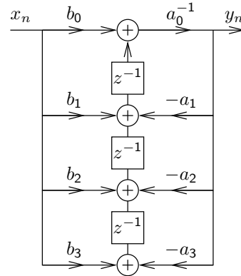
Transposed direct form II:
