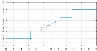
Non-uniform quantization:
