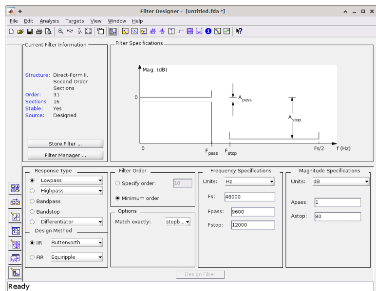
MATLAB Filter Designer
