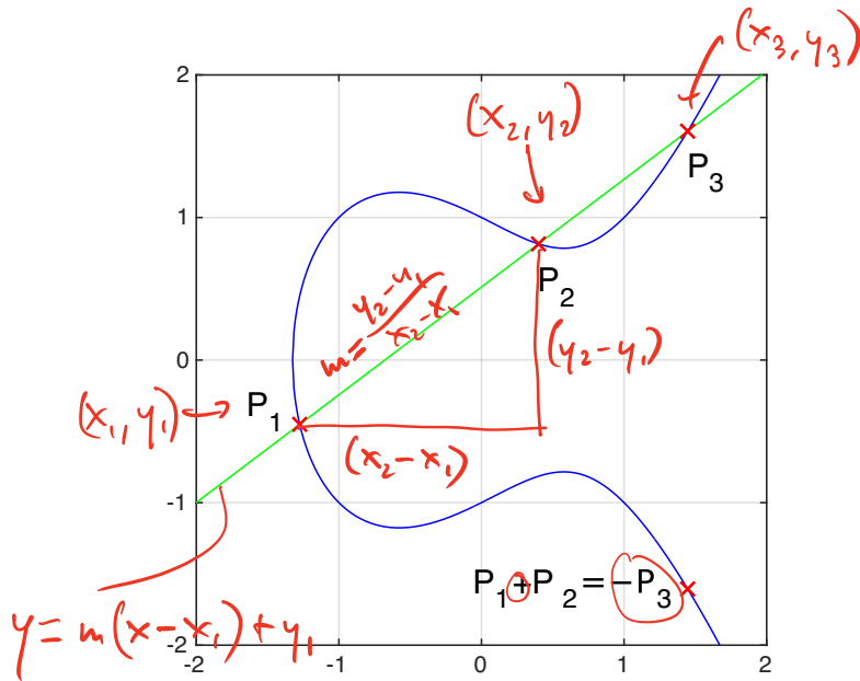
elliptic curve over \mathbb{R} ( a = -1, b = 1 )
