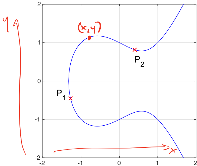
elliptic curve over \mathbb{R} ( a = -1, b = 1 )
