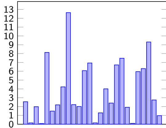
shifted letter freq. (IC=0.065)
