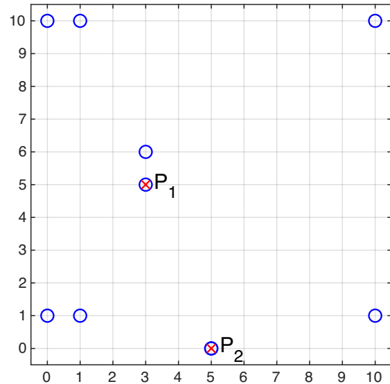
elliptic curve over \mathbb{Z}_{11} ( a = -1, b = 1 )
