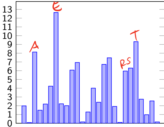
shifted letter freq. (IC=0.065)
