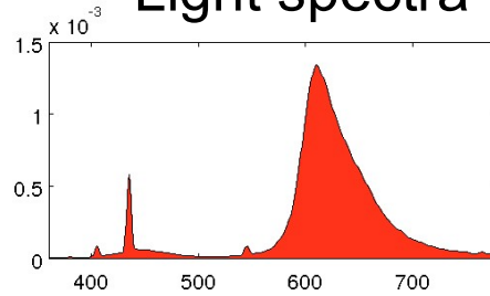
Light spectra
