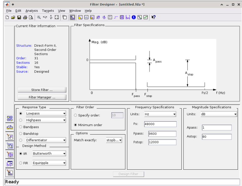
MATLAB Filter Designer
