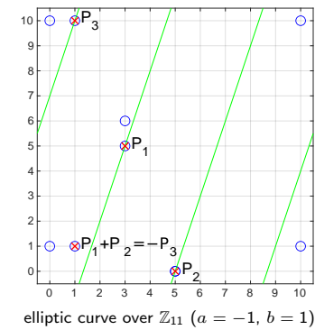
elliptic curve over \mathbb{Z}_{11} ( a = -1, b = 1 )
