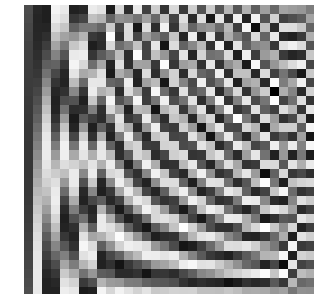
Matrix U with eigenvector columns
