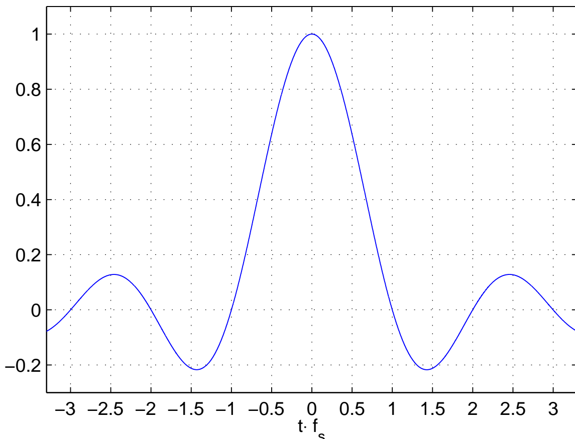
Impulse response of rectangular filter with cut-off frequency f_s/2
