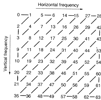
Zigzag ordering of DCT coefficients
