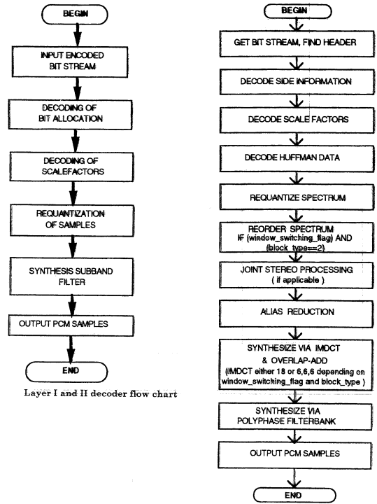
Layer III decoder flow chart
