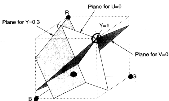
Relationship between the RGB and YUV coordinate systems
