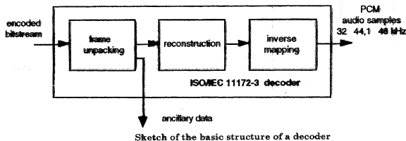
Sketch of the basic structure of a decoder
