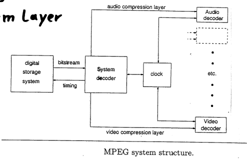
MPEG system structure.
