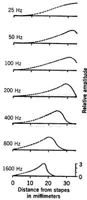
Envelopes of vibrations for various frequencies over the basilar membrane in human cadaver. The maximum displacement amplitude moves toward the stapes as frequency is increased.
