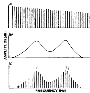
Idealized spectra showing that when the complex vocal waveform (a) is passed through the vocal tract filters (b) the resulting waveform (c) represents the acoustic characteristics of the vocal tract. Vocal tract resonances result in the formants (F 1 , F 2 ).
