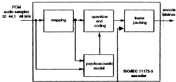
Sketch of the basic structure of an encoder
