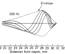
Various momentary positions within a cycle and the envelope formed of a traveling wave along the basilar membrane for a tone of 200 Hz.
