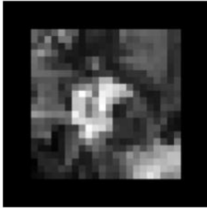
zero
