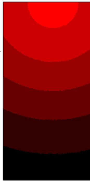
8-bit gradient
