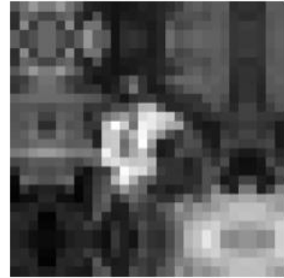
mirror
