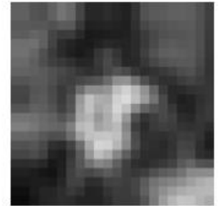
mirror
