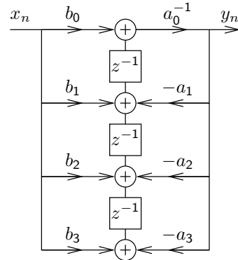
Transposed direct form II:
