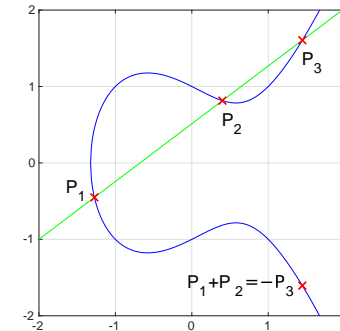
elliptic curve over \mathbb{R} ( A = -1, B = 1 )
