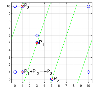
elliptic curve over \mathbb{Z}_{11} ( A = -1, B = 1 )
