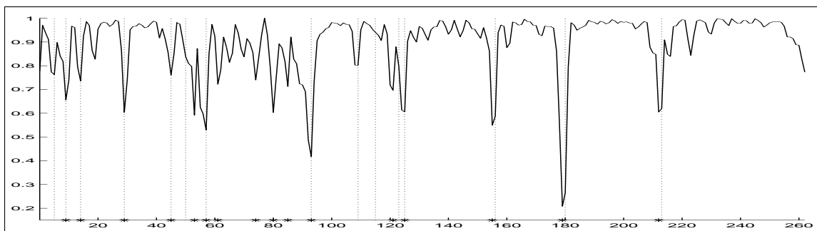
Figure 1: Application of the LCseg algorithm on the concatenation of 16 WSJ stories. Numbers on the x-axis represent sentence indices, and y-axis represents the lexical cohesion function. The representative example presented here is segmented by LCseg with an error of P_k = 15.79 , while the average performance of the algorithm is P_k = 15.31 on the WSJ test corpus (unknown number of segments).
