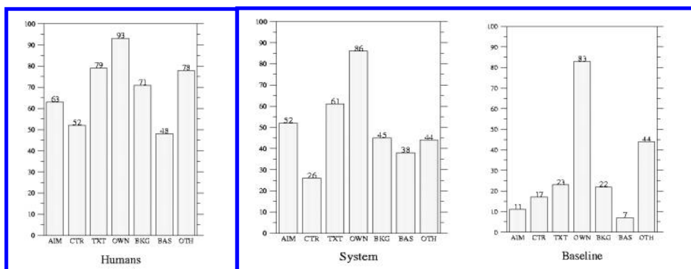
Figure 11 Performance per category: F -measure.
