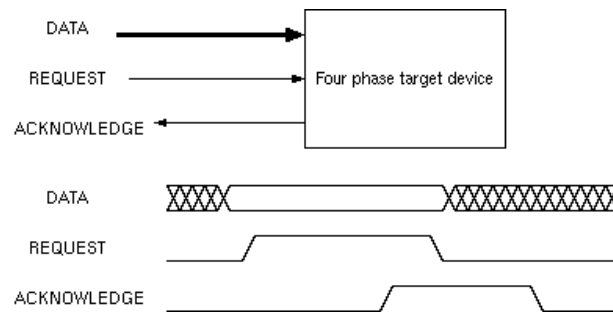
Figure 1.38: Timing diagram for an asynchronous, four-phase handshake.
