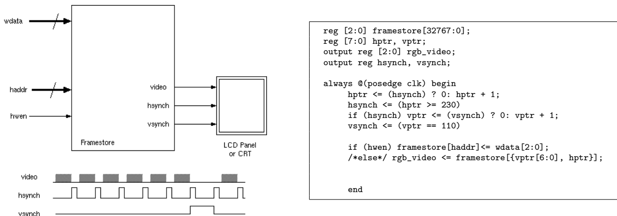
Figure 1.18: Super video graphics adaptor (SVGA) analog framestore output port.
