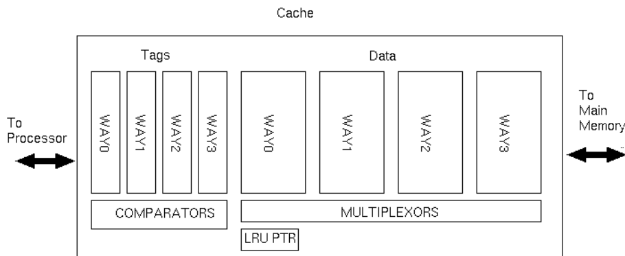
Figure 1.30: Memory blocks and tag comparator needed for a 4-way, set-associative cache.
