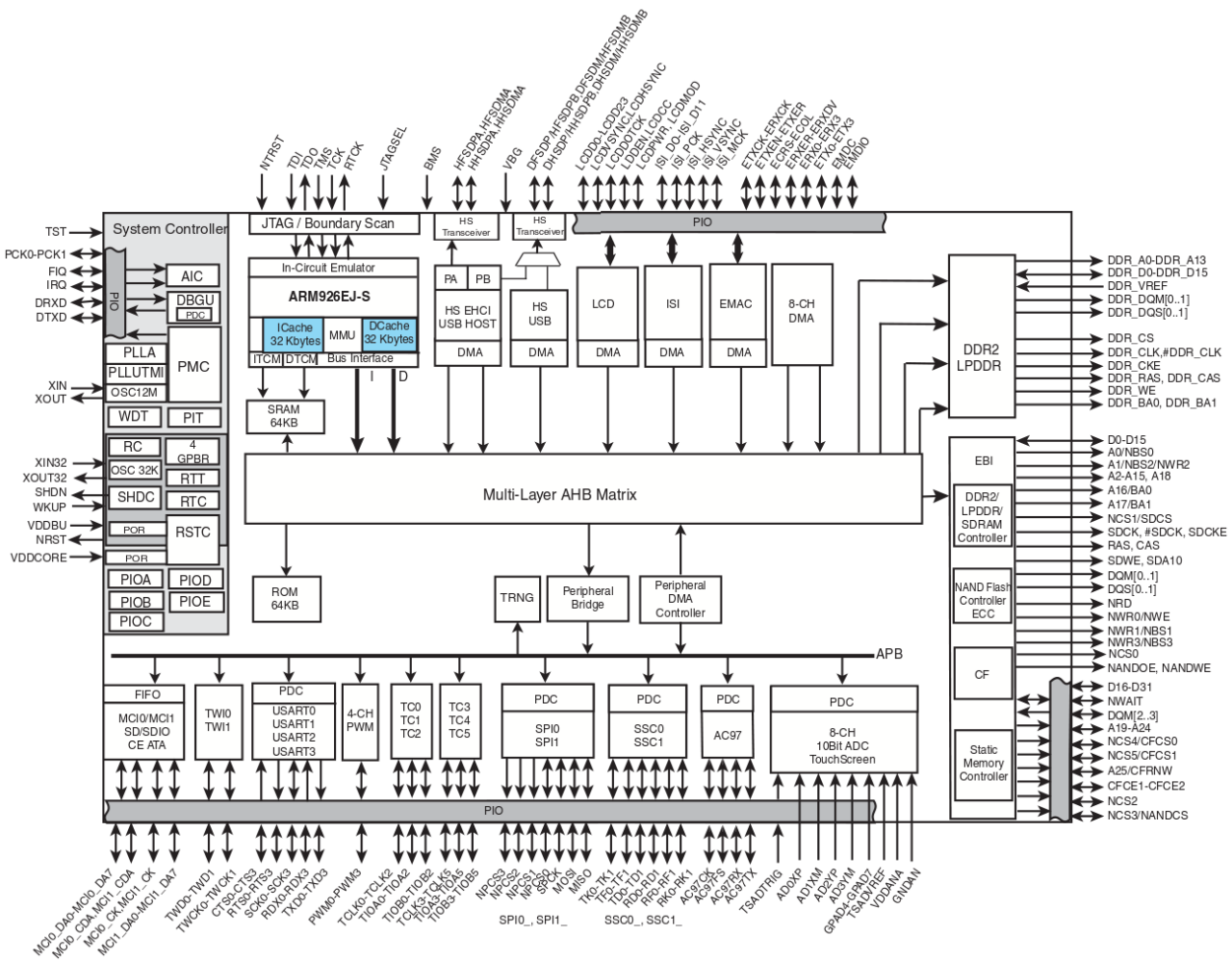
Figure 1.33: Platform Chip Example: Atmel SAM Series 9645.
