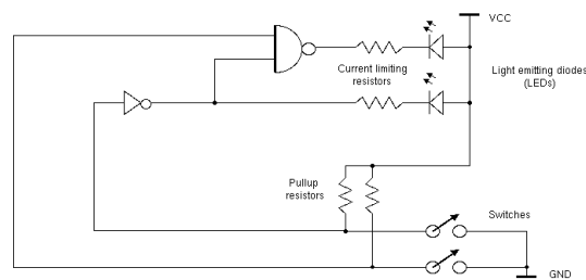
Figure 1.7: Connecting LEDs and switches to digital logic.
