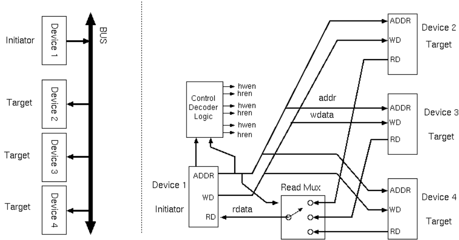
Figure 1.15: A basic SoC bus structure where one initiator addresses three targets (macroview and detailed wiring).
