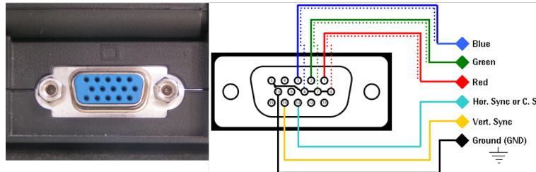
Figure 1.18: Super video graphics adaptor (SVGA) analog framestore output port.
