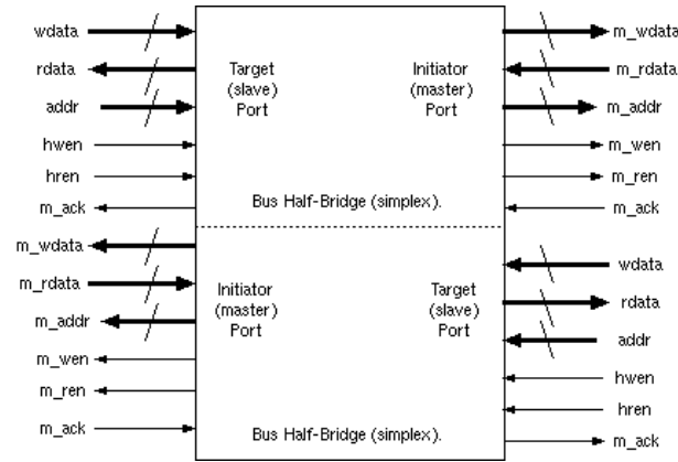
Figure 1.22: Bi-directional bus bridge, composed from a pair of back-to-back simplex bridges.
