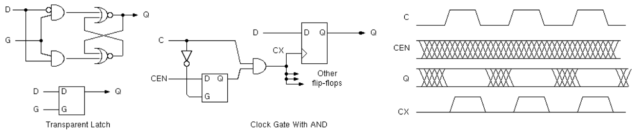
Figure 2.11: Illustrating a transparent latch and its use to suppress clock gating glitches.
