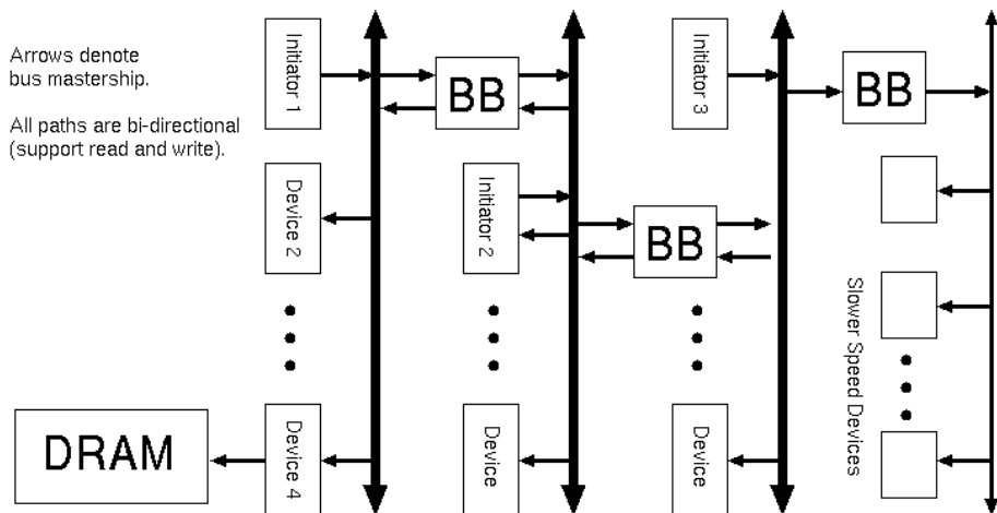
Figure 1.37: A system design using three main busses.
