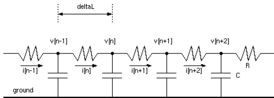
Figure 4.11: Baseline finite-difference model for bidirectional propagation in one dimension.
