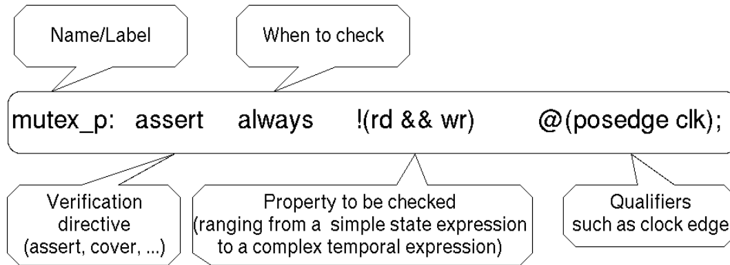
Figure 5.3: General structure of a PSL assertion
