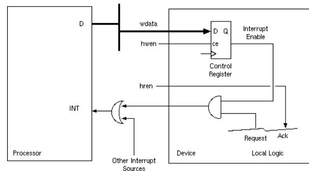
Figure 1.17: Interrupt generation: general structure within a device and at system level.
