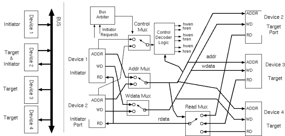
Figure 1.19: SoC bus structure where one of the targets is also an initiator (e.g. a DMA controller).
