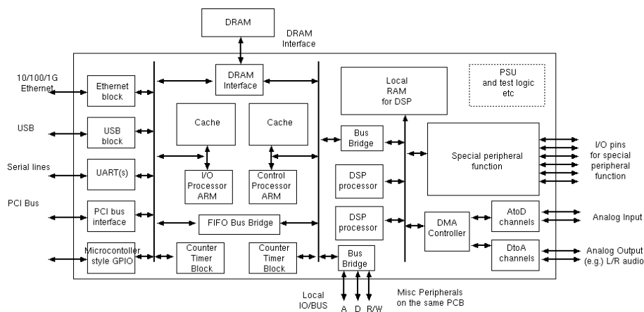
Figure 1.31: Platform Chip Example: Virata Helium 210
