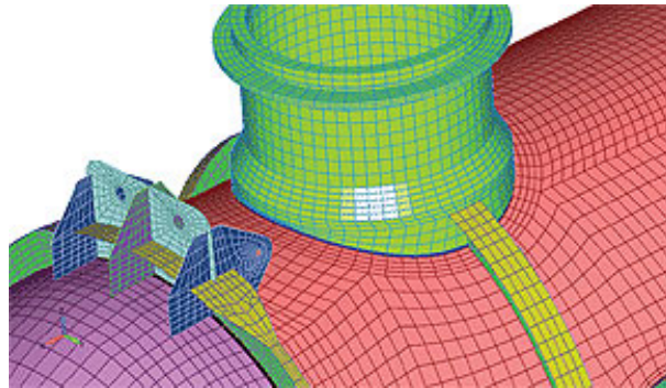
Figure 4.10: Finite Element Grid
