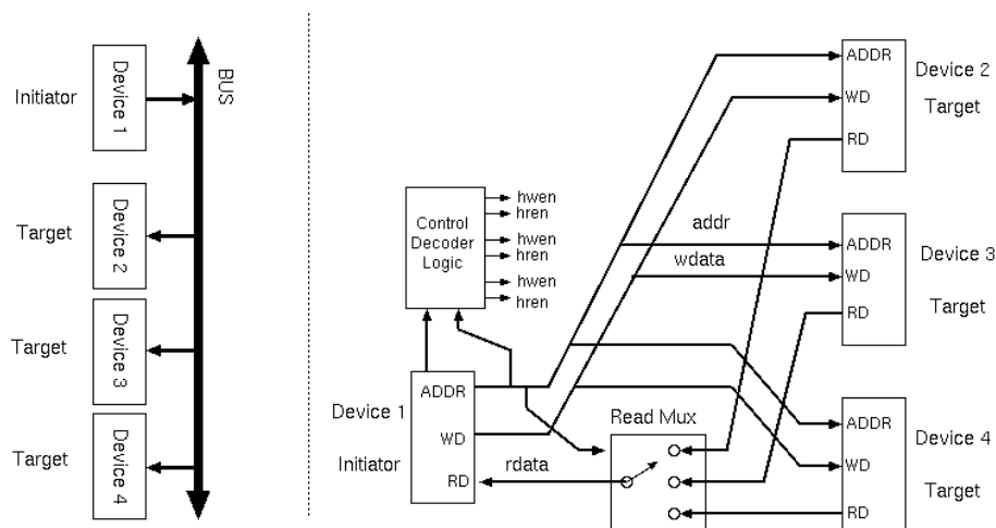
Figure 1.35: Example where one initiator addresses three targets.
