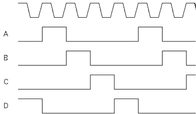
Figure 5.4: Desired behaviour of the four nets.
