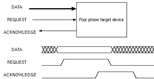
Figure 1.14: Timing diagram for an asynchronous, four-phase handshake.
