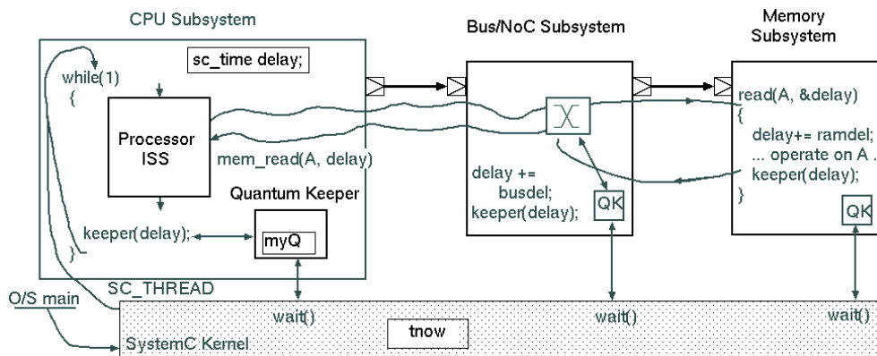
Figure 7.8: Typical setup of thread using loosely-timed modelling with a quantum keeper.
