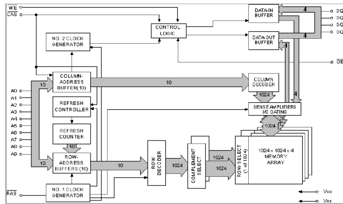
Figure 1.28: Single-bank DRAM Chip Internal Block Diagram.
