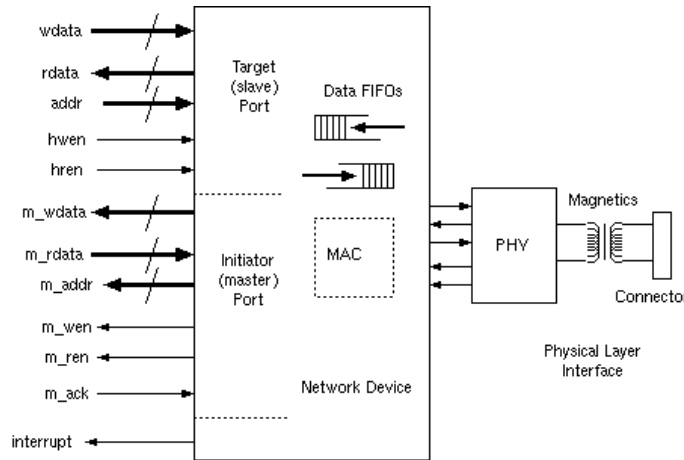
Figure 1.20: Connections to a DMA-capable network device.
