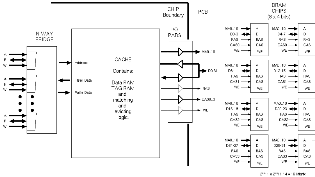
Figure 1.29: Typical structure of a small DRAM subsystem.
