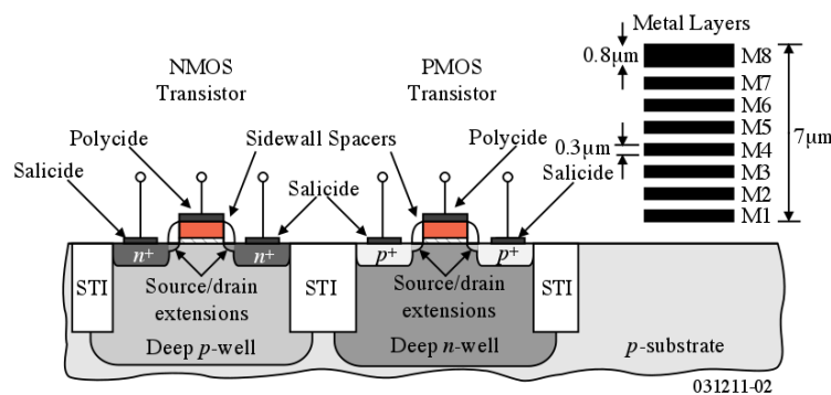
Figure 2.6: Schematic of transistor construction on silicon wafer.
