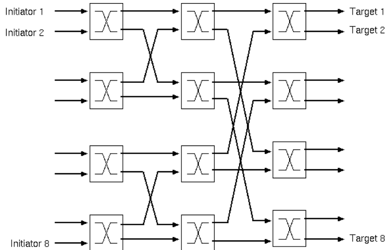
Figure 1.41: A more-complex switching fabric: more wiring, more bandwidth and less fabric contention than ring (but still has output port contention).
