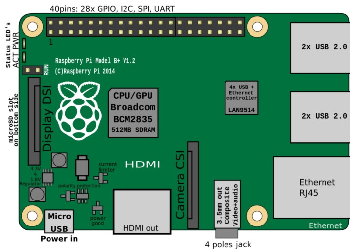
Figure 1.26: Raspberry Pi (Model B) PCB Layout.
