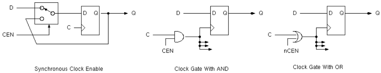
Figure 2.10: Clock enable using multiplexor, AND and OR gate.
