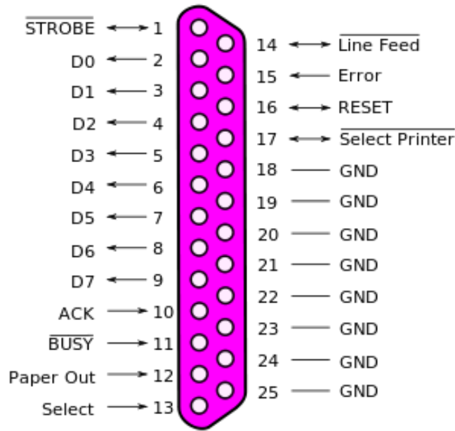
Figure 1.13: (Centronix) Parallel Port Pin Connections
