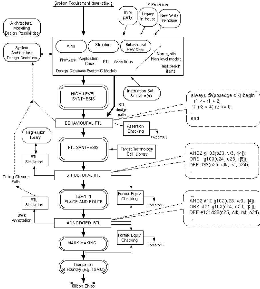
Figure 4.20: Design and Manufacturing Flow for SoC.
