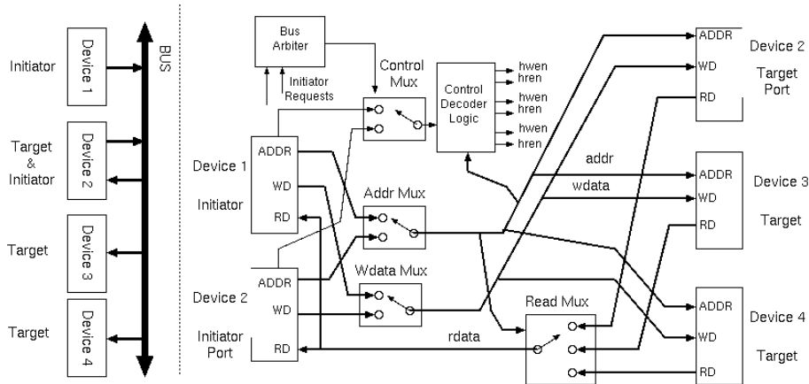
Figure 1.36: Example where one of the targets is also an initiator (e.g. a DMA controller).
