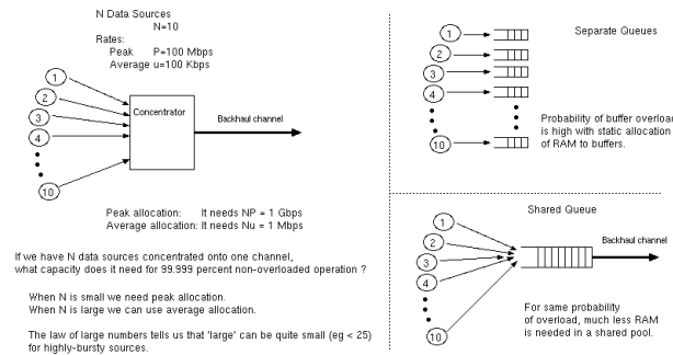
Figure 1.21: Extra diagram illustrating statistical muxlplexing gain [Non-examinable].
