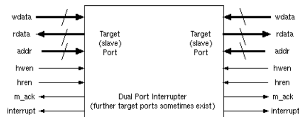
Figure 1.23: Dual-port interrupter (doorbell) or mailbox.
