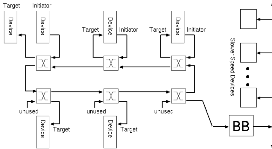
Figure 1.40: A ring network: a low-complexity network on chip structure.
