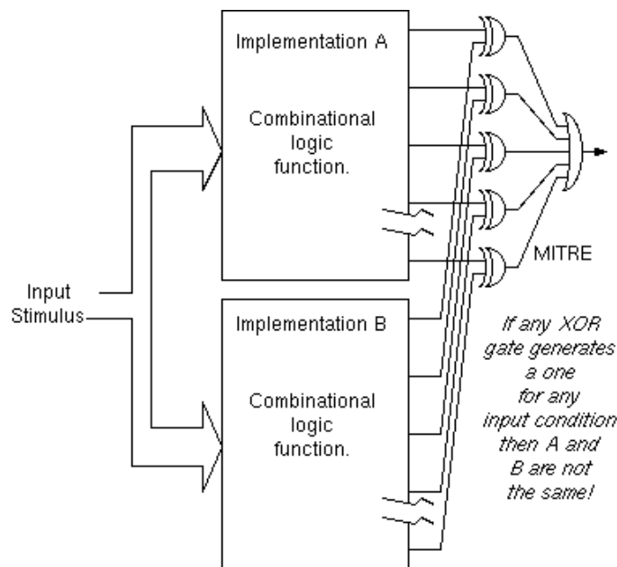
Figure 5.5: A mitre compares the outputs from a pair of supposedly-equivalent combinational components.
