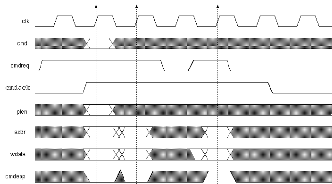
Figure 1.39: BSCI Protocol, Command Timing Diagram
