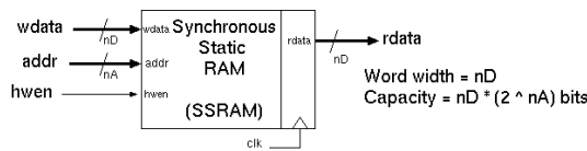
Figure 1.16: Static RAM with single port.
