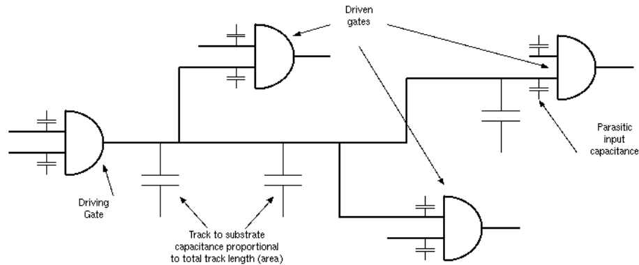
Figure 2.3: Logic net with tracking and input load capacitances illustrated.
