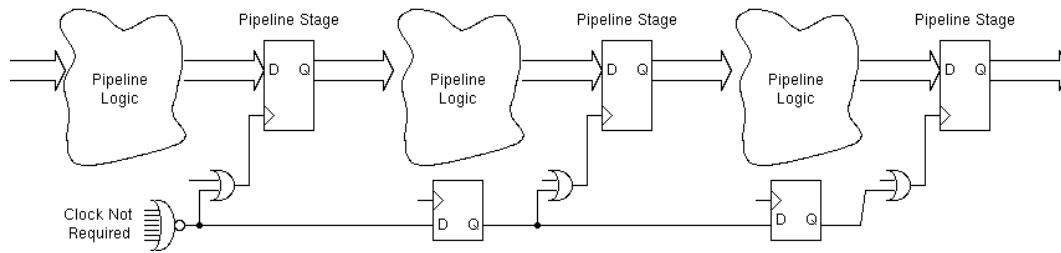
Figure 2.13: Clock needed computations forwarded down a pipeline.
