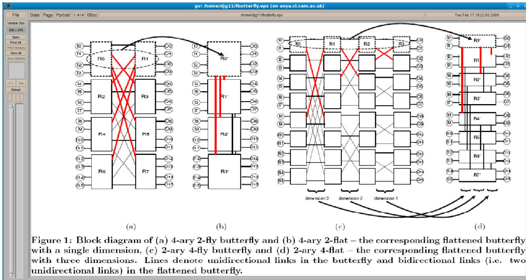
Figure 1.42: The 'Flattened Butterfly' network topology.
