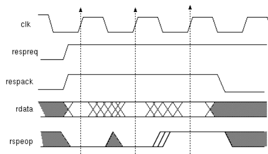
BSCI Response Portion Protocol Timing Diagram
