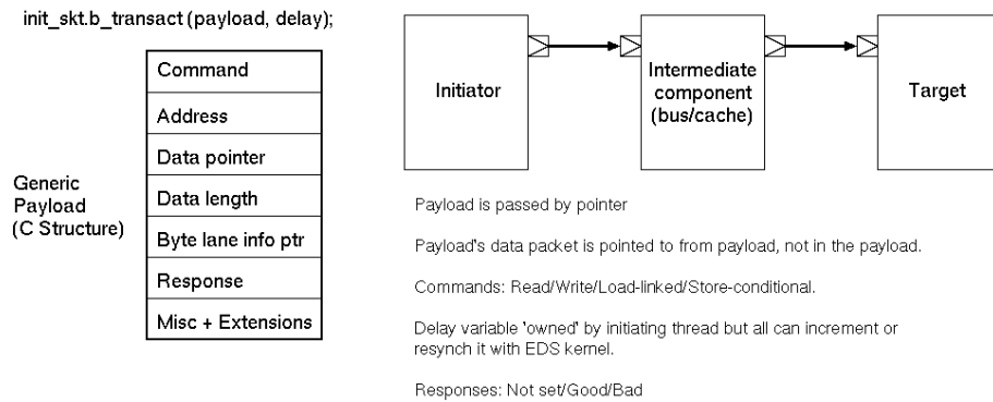
Figure 7.7: The general TLM 2.0 Setup
