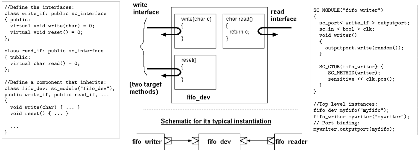
Schematic for the FIFO device:
