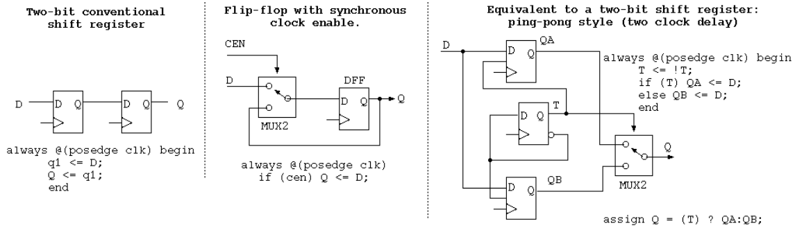
Figure 5.6: Two circuits that use different amounts of internal state to achieve the same functionality.
