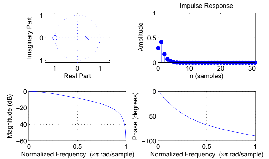
order: 1, cutoff frequency (-3 dB): 0.25 \times f_s/2
