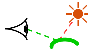
reflection
