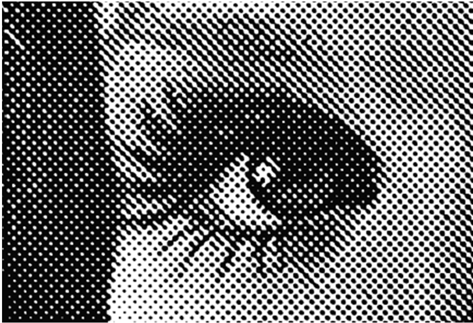
Halftoning
