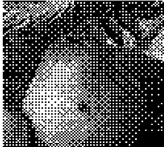
ordered dither
