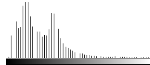
improved histogram
