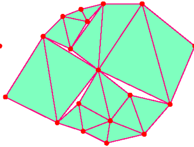
Naïve triangulation
