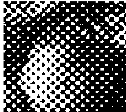
halftoning (5×5 cells)
