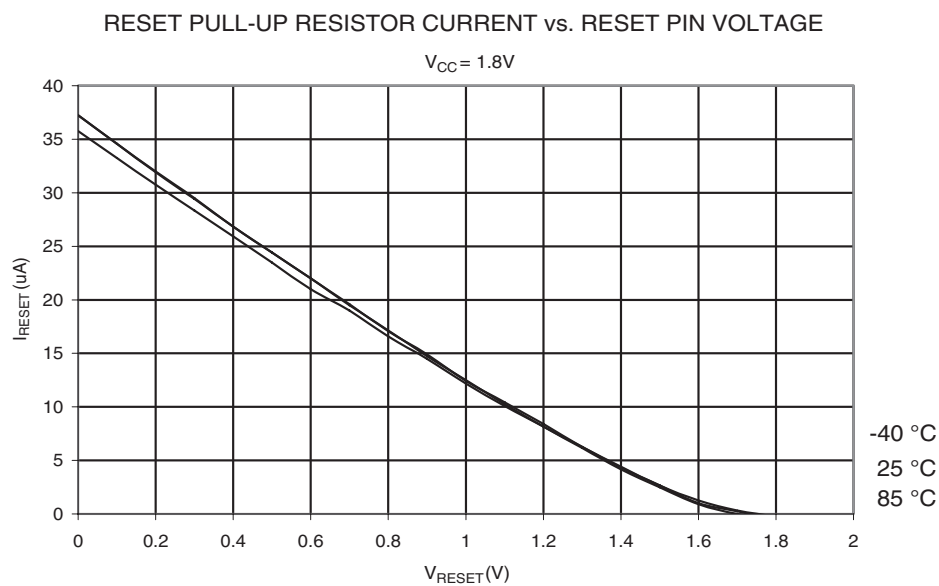
Figure 28-112. Reset Pull-up Resistor Current vs. Reset Pin Voltage ( V_{CC} = 1.8V ).
