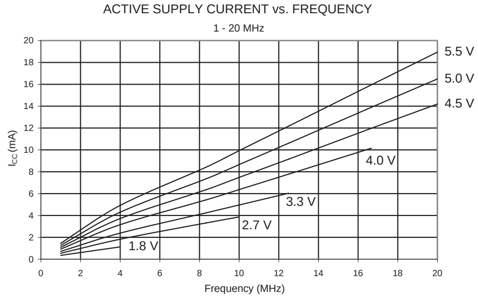
Figure 28-2. Active Supply Current vs. Frequency (1 - 20 MHz).
