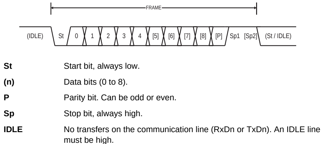
Figure 18-4. Frame Formats
