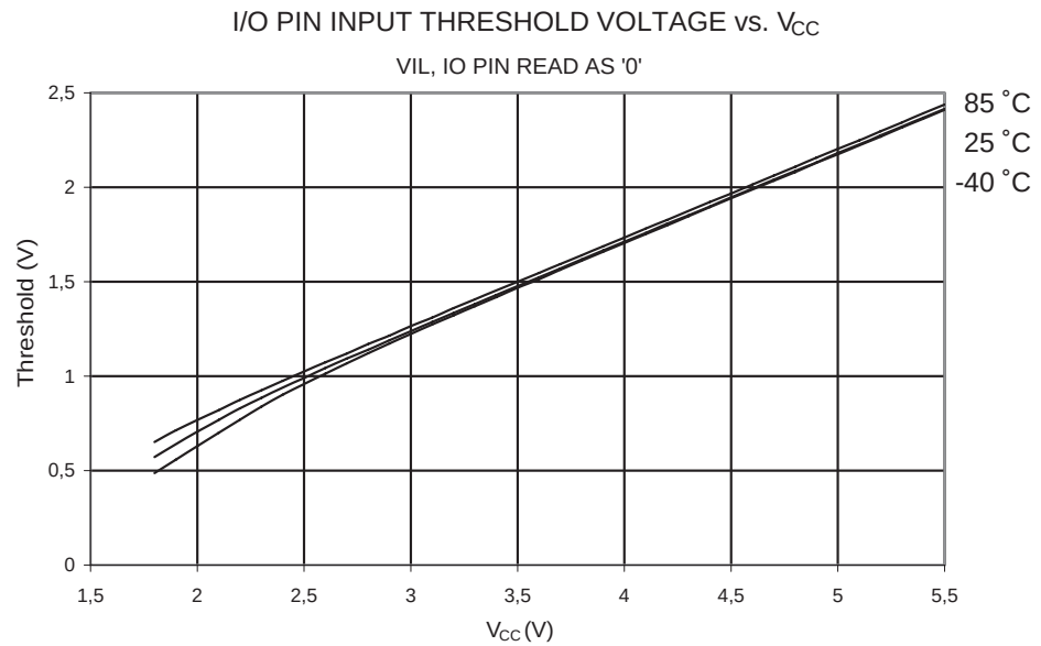
Figure 28-73. I/O Pin Input Threshold vs. V_{CC} ( V_{IL} , I/O Pin Read as '0').
