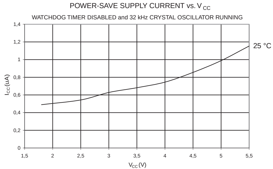
Figure 28-13. Power-save Supply Current vs. V_{CC} (Watchdog Timer Disabled and 32 kHz Crystal Oscillator Running).
