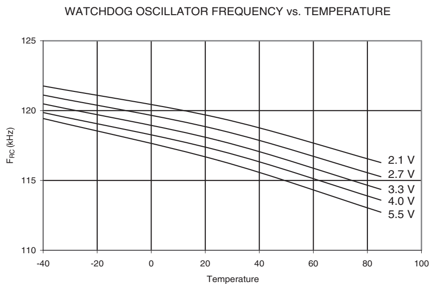
Figure 28-128. Watchdog Oscillator Frequency vs. Temperature
