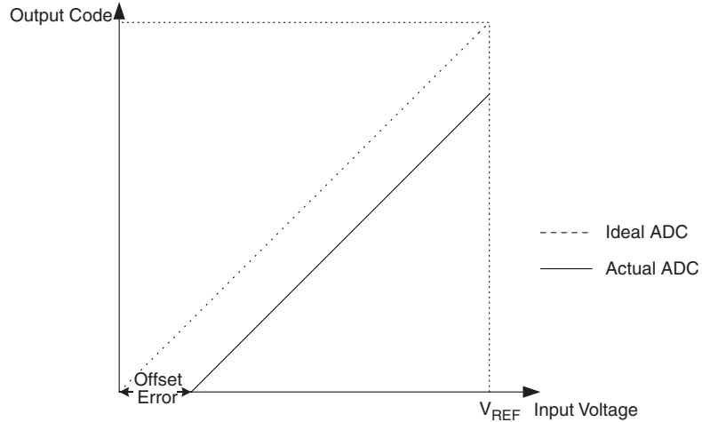
Figure 22-10. Offset Error
