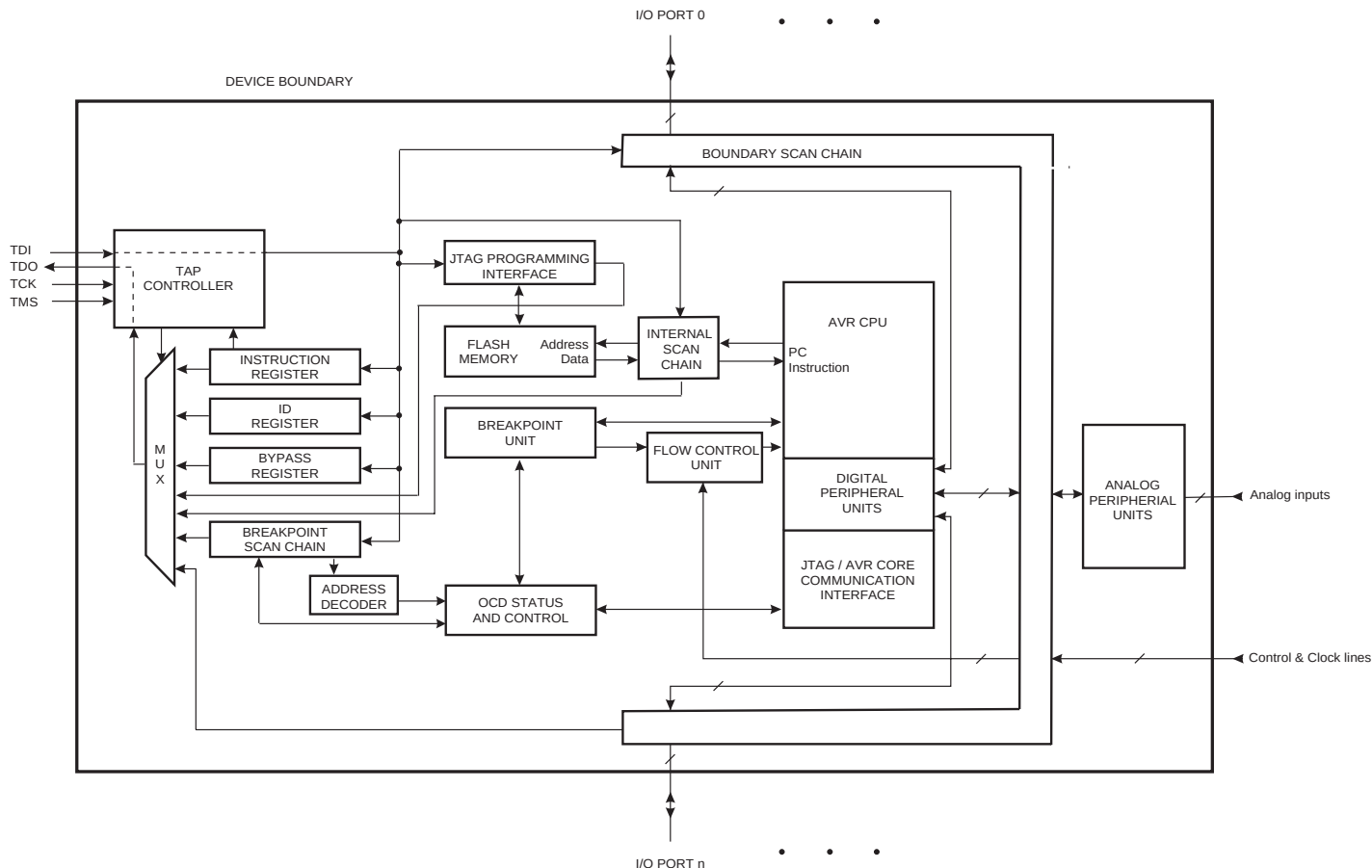
Figure 23-1. Block Diagram
