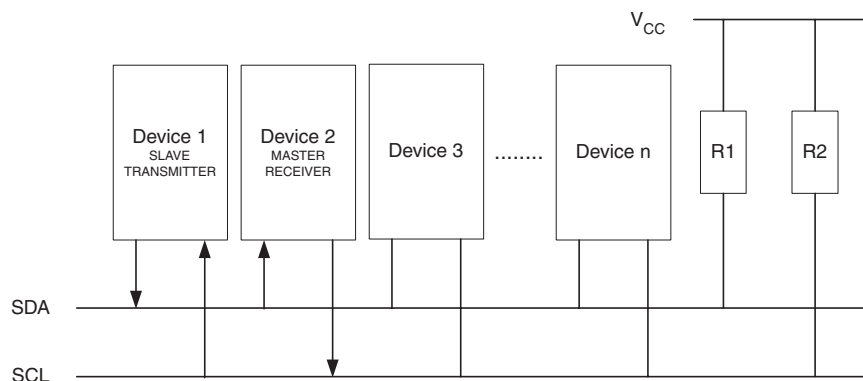
Figure 20-17. Data Transfer in Slave Transmitter Mode
