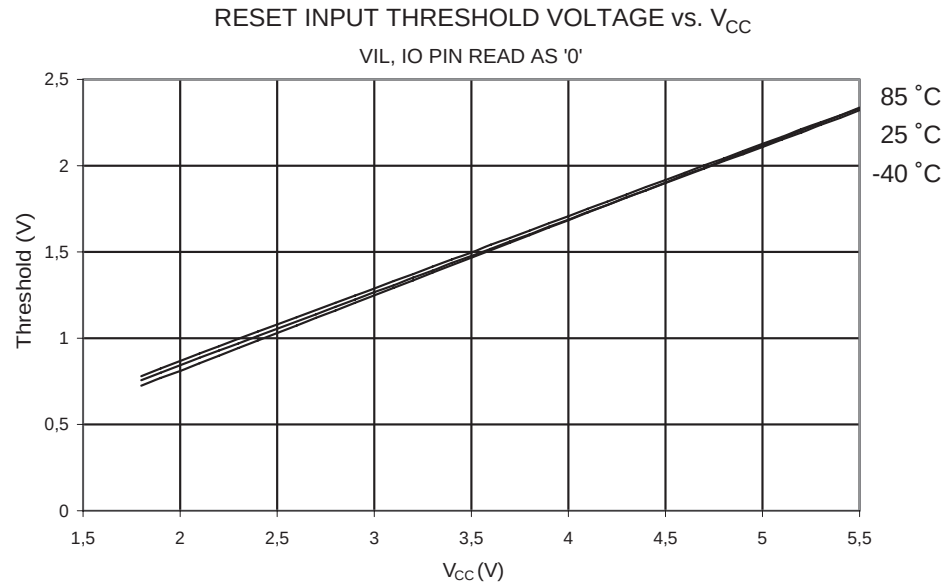
Figure 28-76. Reset Pin Input Threshold vs. V_{CC} ( V_{IL} , I/O Pin Read as '0').
