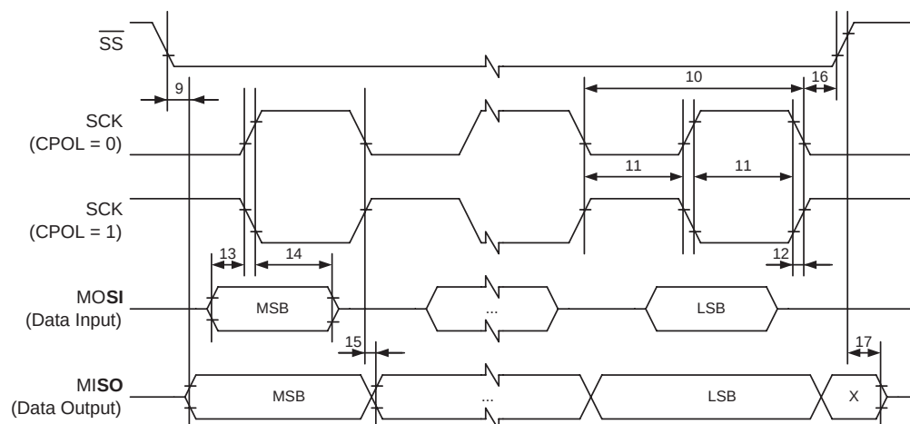
Figure 27-5. SPI Interface Timing Requirements (Slave Mode)
