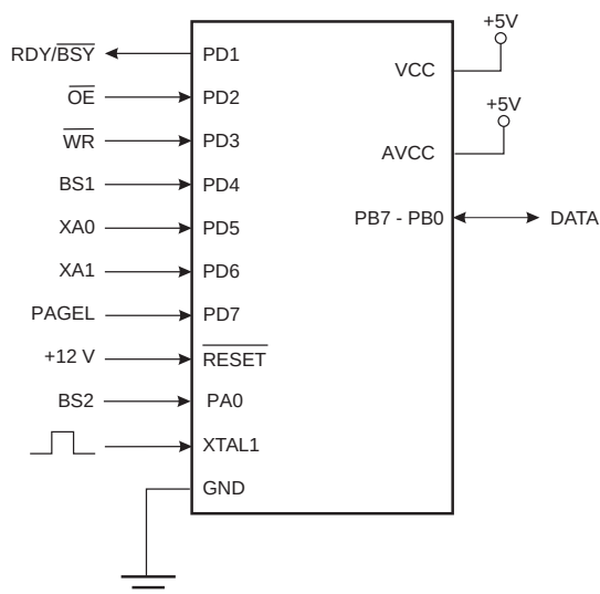
Figure 26-1. Parallel Programming (1)
