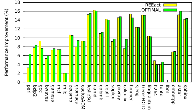
Figure 4. Performance (execution time) improvement of SPEC with REEact broken-screw policy and manually tuned optimal execution, compared to the Linux default scheduler.
