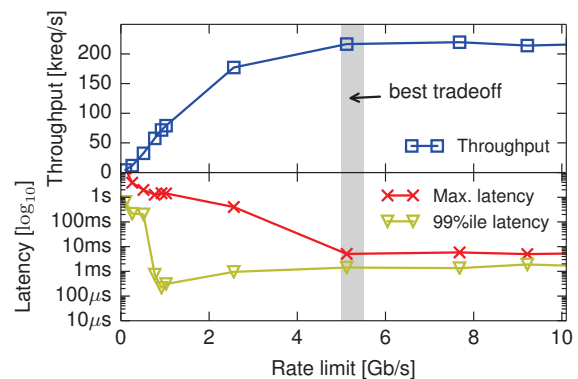
Figure 10: memcached throughput (top) and latency (bottom, \log_{10} ) as a function of the QJUMP rate limit.
