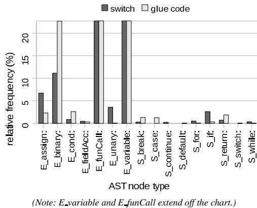
Figure 5. AST node frequencies in glue and non-glue code
