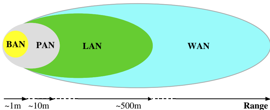
Figure 1. Networks Taxonomy
