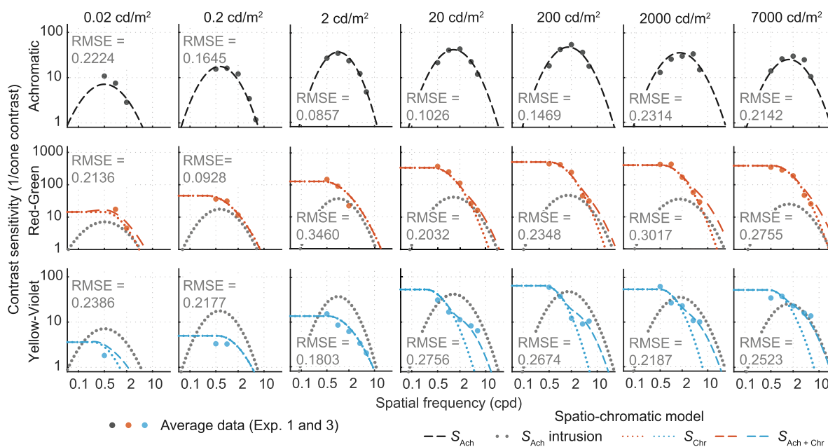
Figure 15. Model predictions including luminance intrusion and parameters as a function of the light level, based on Equations 13 to 16.
