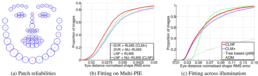
Figure 4: a) The reliabilities of CLNF patch experts, smaller circles represent more reliability (less variance). b) Fitting on the Multi-PIE dataset, observe the performance boost from both the LNF patch expert and the NU-RLMS fitting method. Their combination (CLNF) leads to the lowest error, since NU-RLMS performs even better on more reliable response maps. c) Fitting on the unseen illumination Multi-PIE subset. Note the good generalisability of CLNF.
