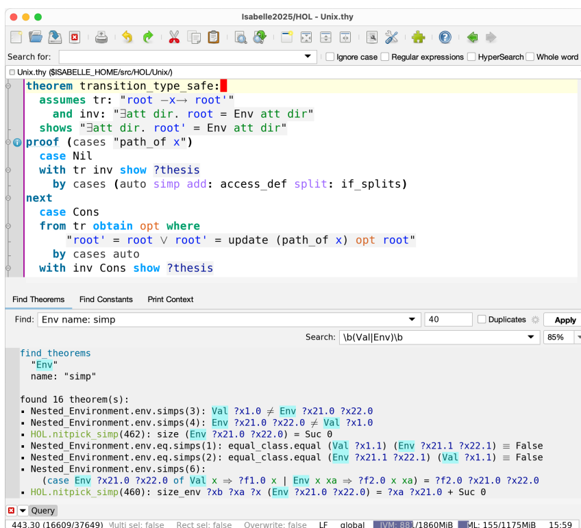
Figure 3.5: An instance of the Query panel: find theorems
