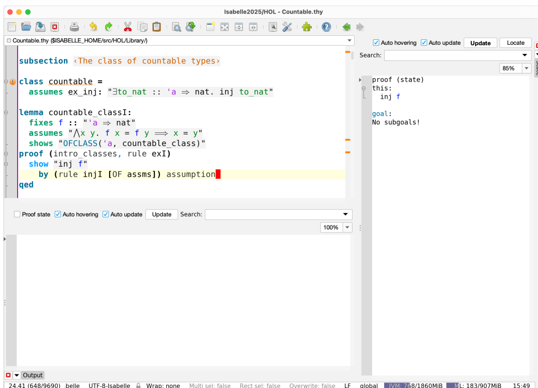
Figure 3.4: Separate proof state display (right) and other output (bottom).
