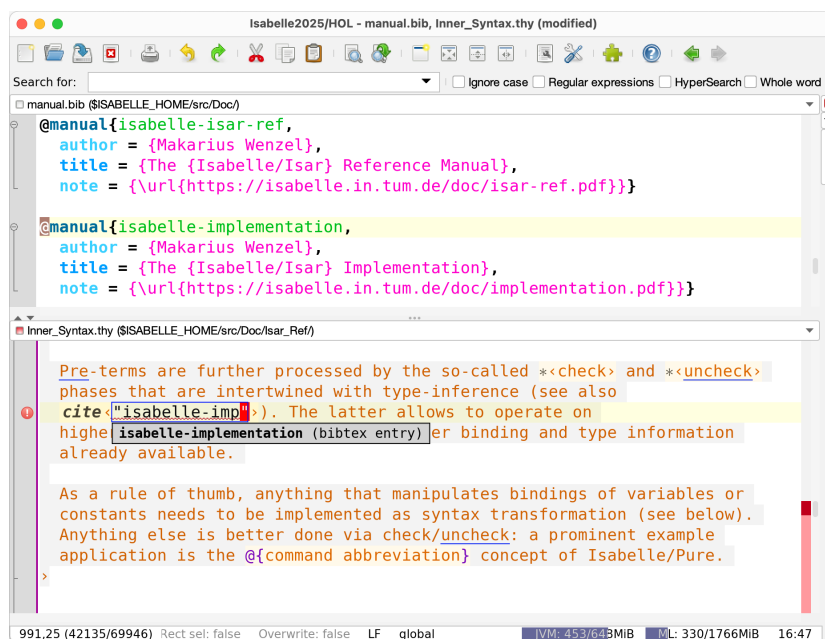
Figure 4.3: Semantic completion of citations from open BibTeX files
