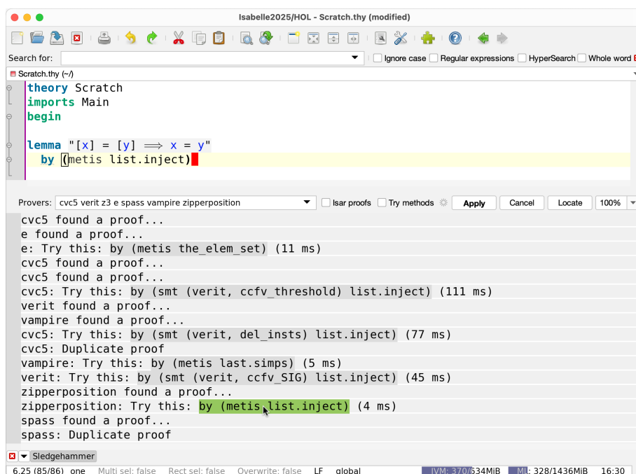
Figure 3.12: An instance of the Sledgehammer panel
