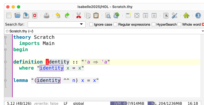
Figure 3.8: Visualized markup for nested infix expressions
