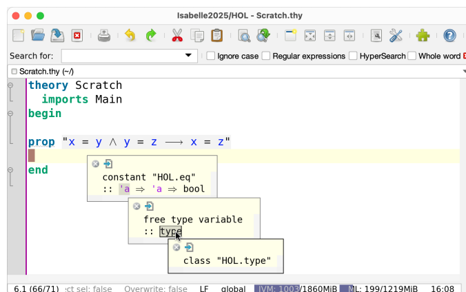
Figure 3.7: Nested tooltips over formal entities
