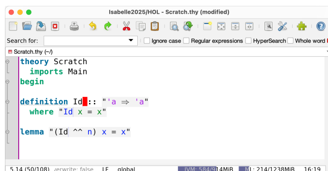
Figure 3.10: The result of semantic selection and systematic renaming
