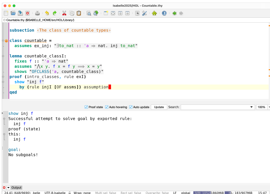
Figure 3.3: Proof state display within the regular output panel
