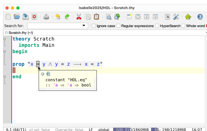
Figure 3.6: Tooltip and hyperlink for some formal entity
