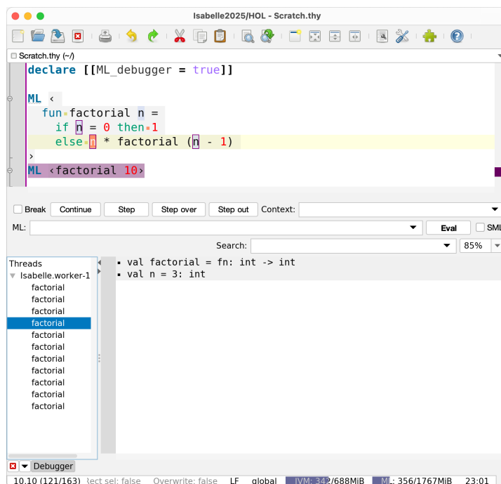
Figure 5.1: ML debugger session
