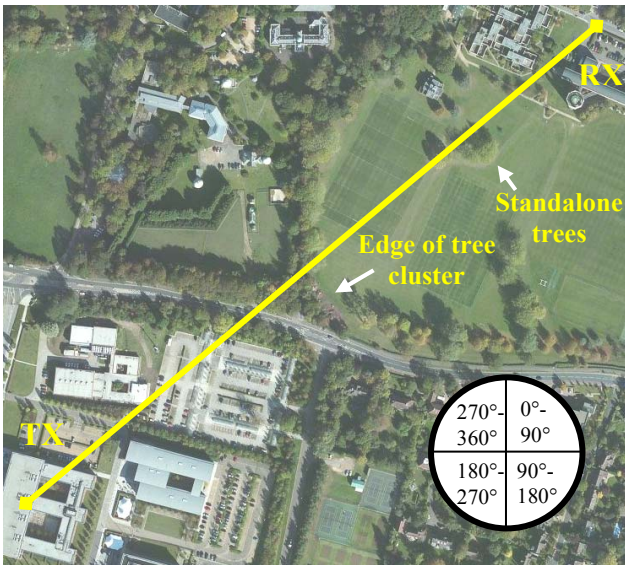
Figure 2: Plan view of Link B.
