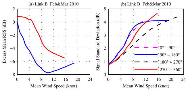
Figure 4: Distribution of excess mean RSS and standard deviation of RSS within 10-minute at different mean wind speed for four mean direction sectors in Link B (Off-leaf). (a) Trends of slow fading (b) Trends of fast fading.
