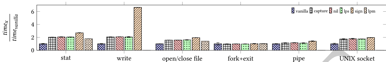
Figure 9: Normalised overhead of queries (LPM capture overhead as reported in [18] is given when available).
