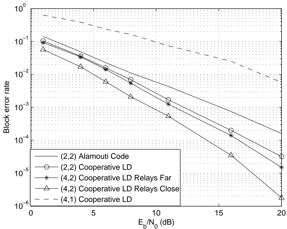
Figure 3: Cooperative LD code optimized in different physical configurations vs Alamouti code for (2,2) system under Rayleigh fading.
